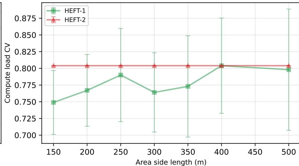
Large DAG — Compute load CV
