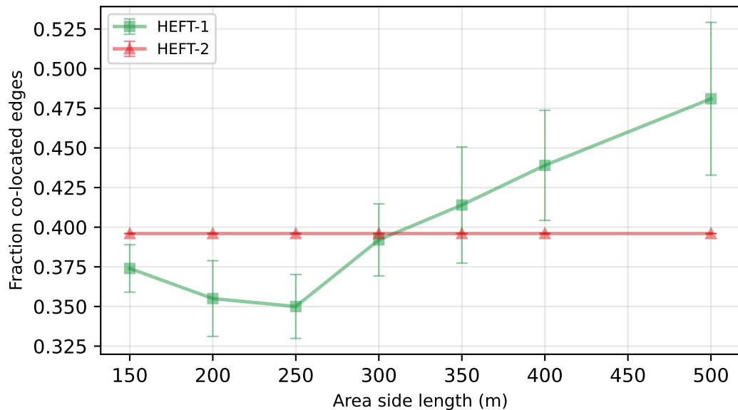
Large DAG — Fraction co-located edges
